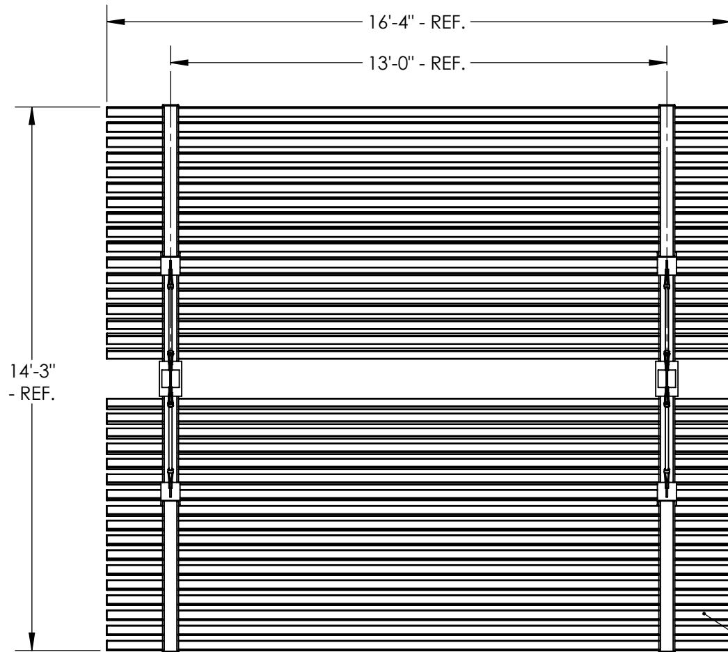
TOP VIEW
