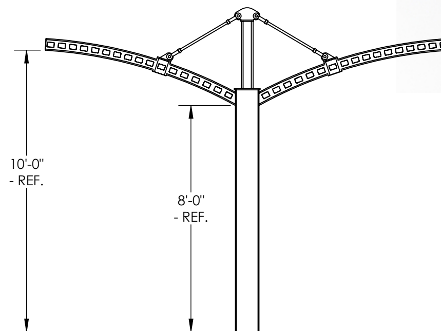
END VIEW
