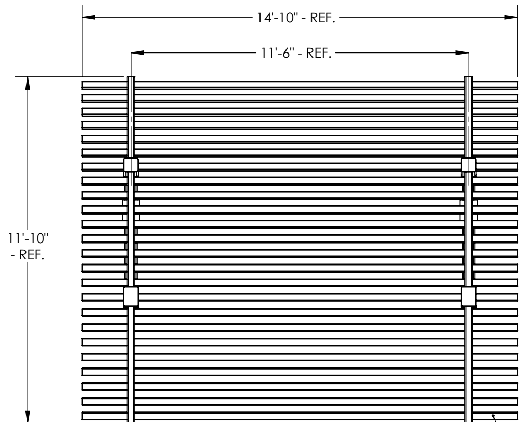
TOP VIEW
