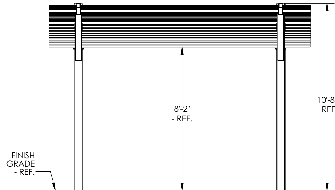
FRONT VIEW
