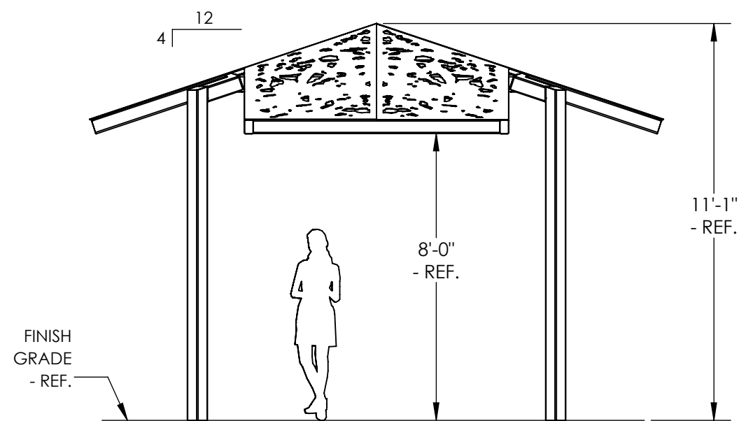
SIDE VIEW
