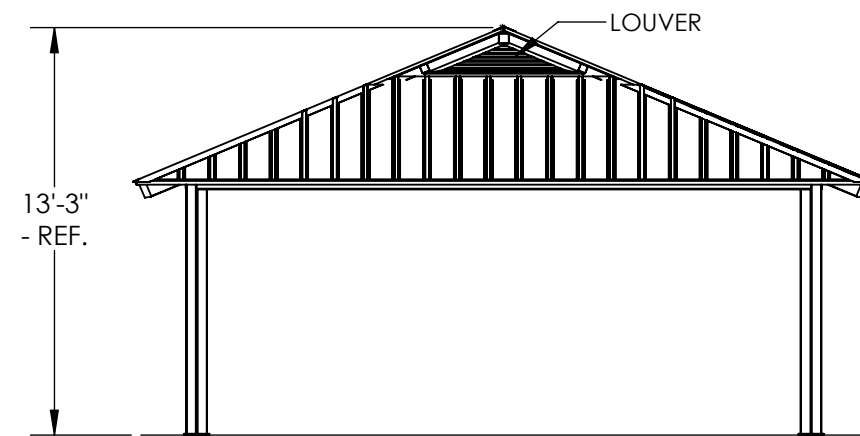
END VIEW
