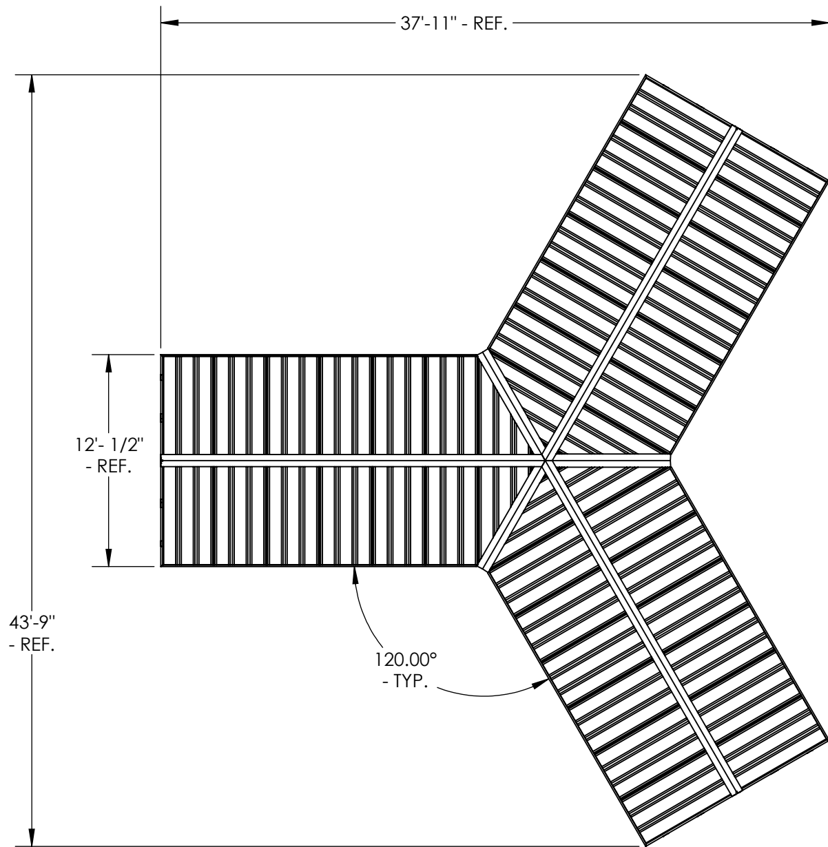
TOP VIEW
