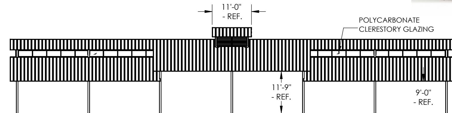
SIDE VIEW
