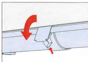
Snap on the gutter connector
